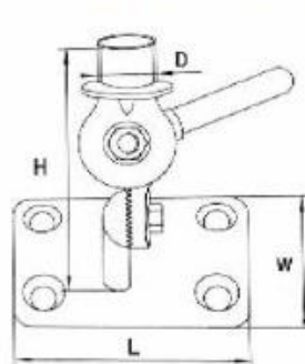
AISI316 STAINLESS STEEL ANTENNA BASE
