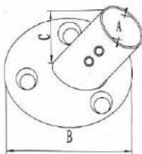
AISI316 STAINLESS STEEL HANDRAIL 60° ROUND BASE
